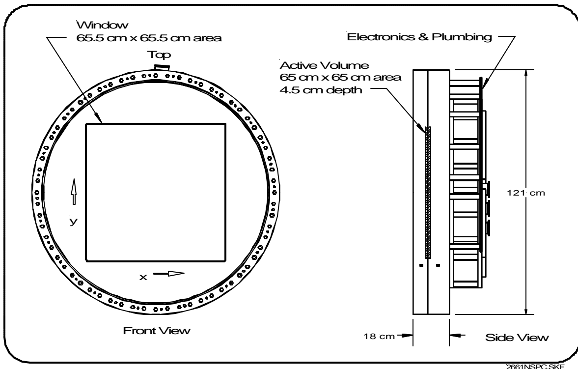
ORDELA Model 2661N outline and dimensions
