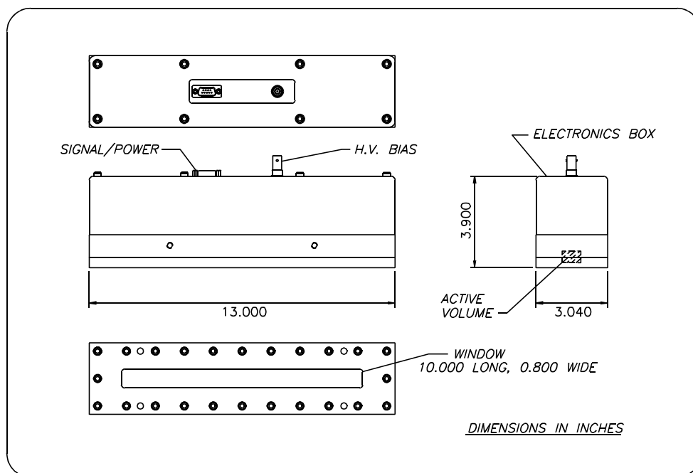
ORDELA MODEL 1250N OUTLINE AND DIMENSIONS
