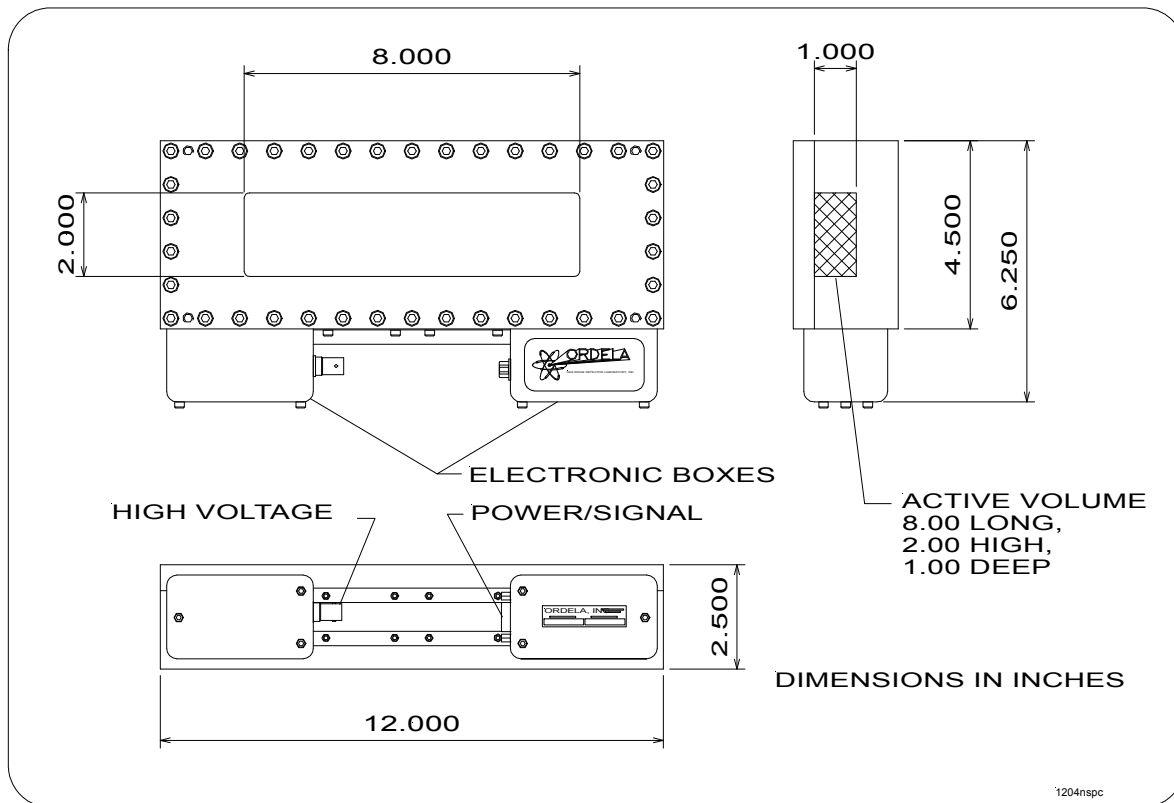
ORDELA Model 1200N, outline and dimensions
