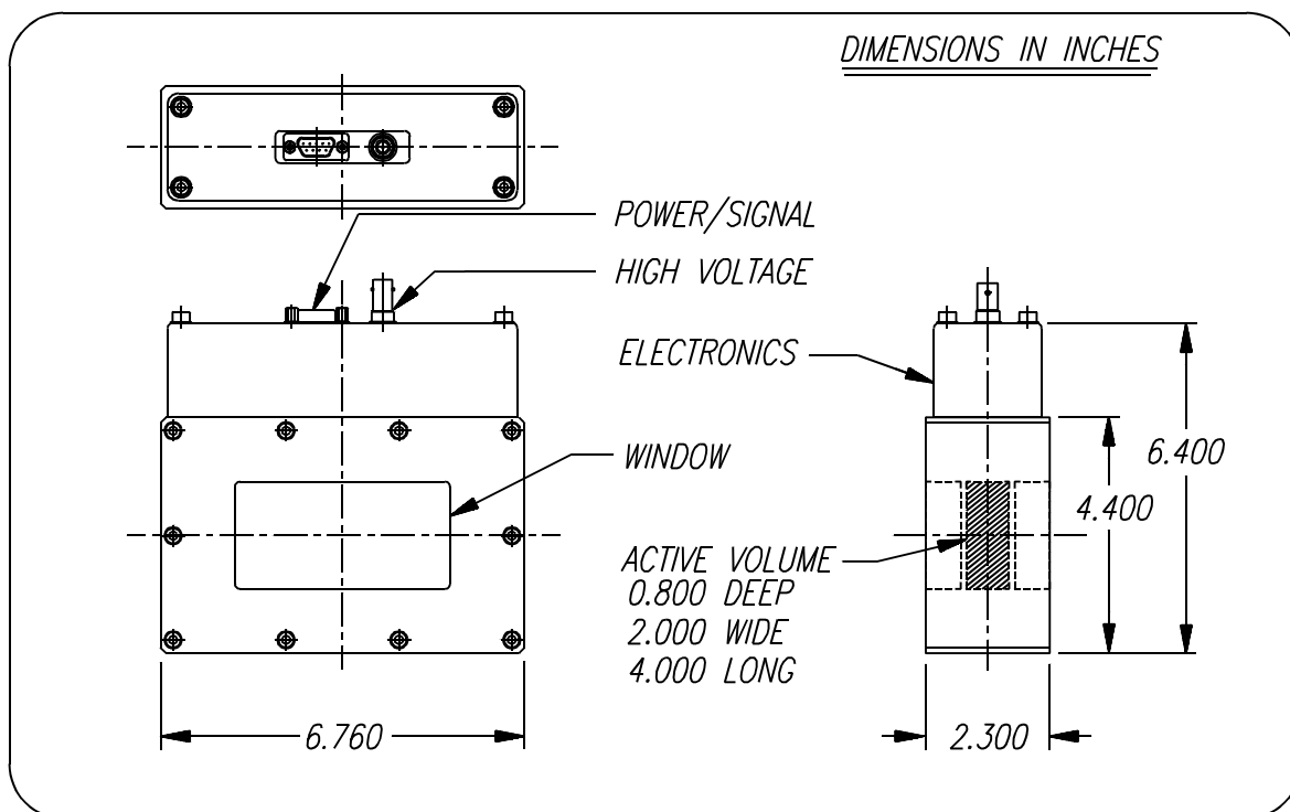
ORDELA MODEL 1150N OUTLINE AND DIMENSIONS
