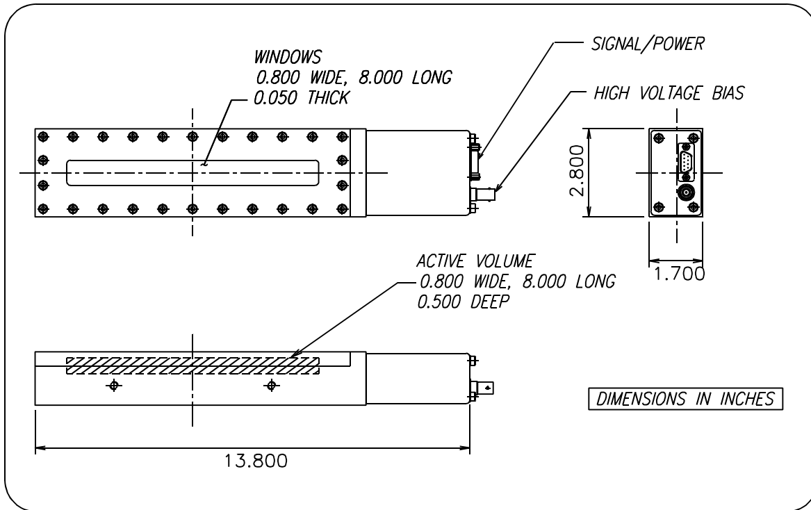
ORDELA MODEL 4220N OUTLINE AND DIMENSIONS
