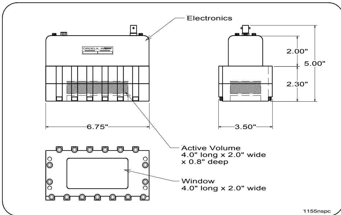
ORDELA MODEL 1155N OUTLINE AND DIMENSIONS
